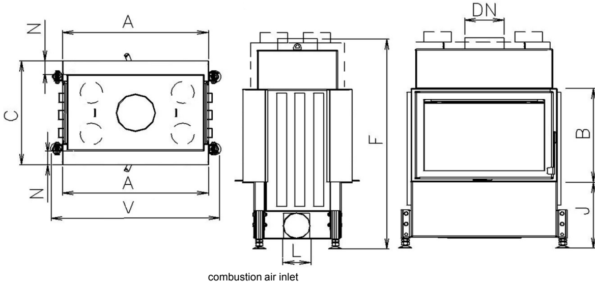
combustion air inlet
