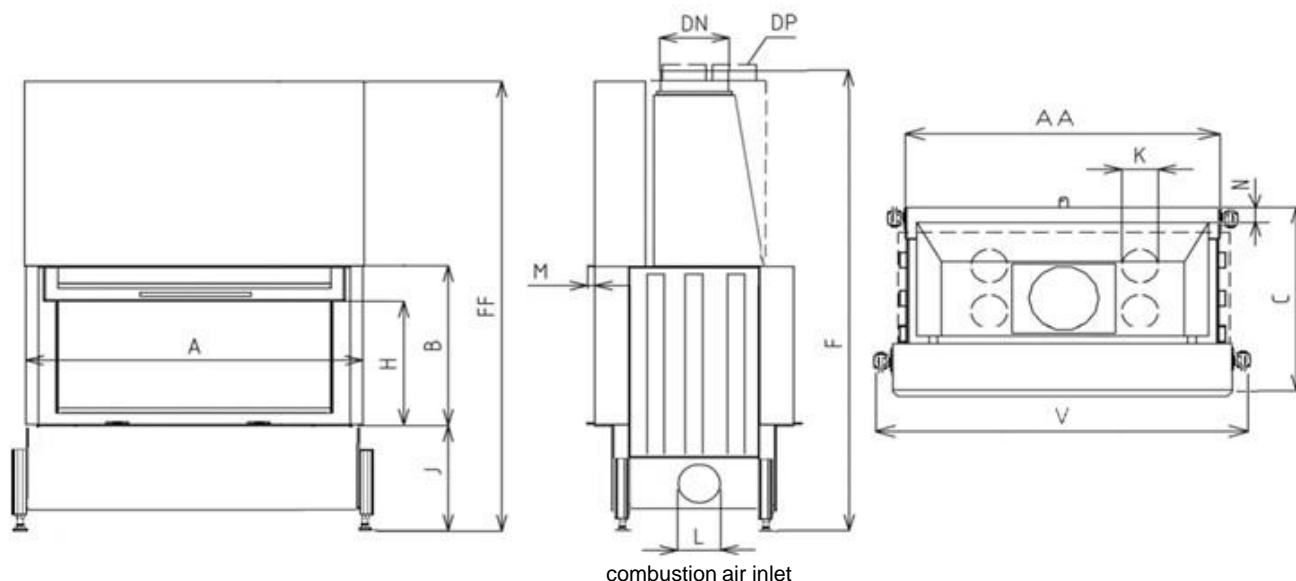
combustion air inlet
